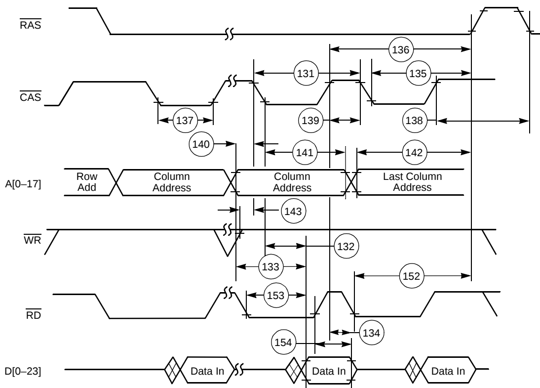
Figure 2-16. DRAM Page Mode Read Accesses
