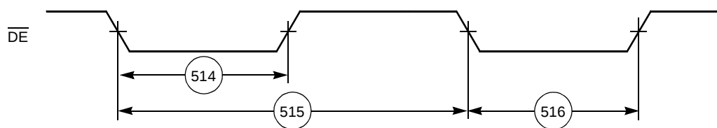
Figure 2-48. OnCE—Debug Request
