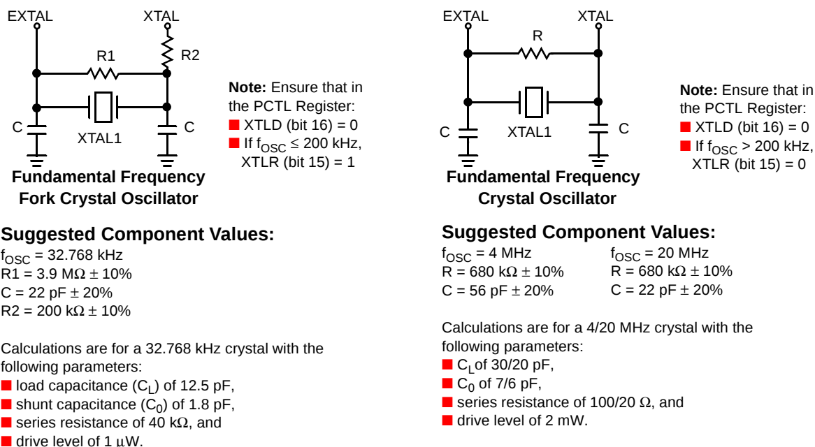
Figure 2-1. Crystal Oscillator Circuits
